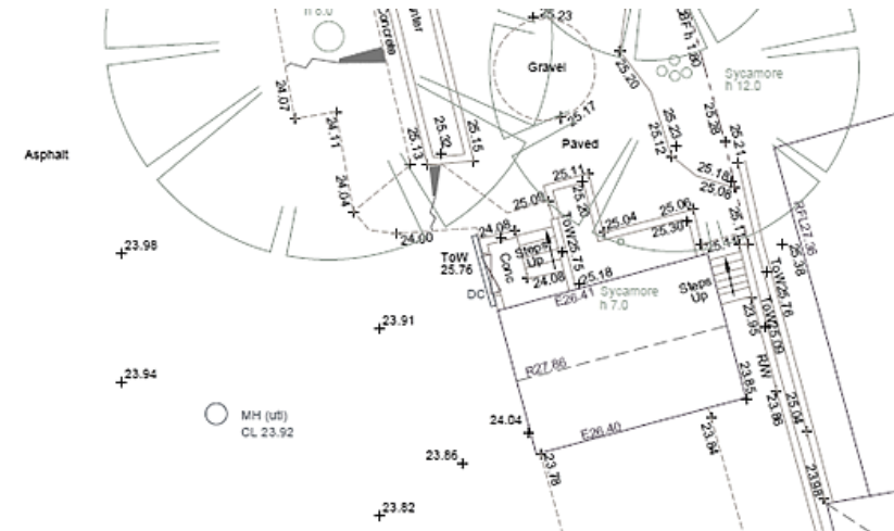
TOPOGRAPHICAL SURVEY EXAMPLE BELOW SHOWING THE LEVEL OF DETAIL AND ACCURACY OF MEASUREMENTS
